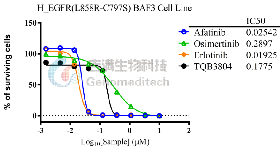
Figure 1 | Cell proliferation assay. The H_EGFR(L858R-C797S) BAF3 Cell Line (Cat. GM-C29678) at a concentration of 1E4 cells/well (96-well format) was treated with serial dilutions of Osimertinib (AZD9291) (Selleck/S7297), Erlotinib (OSI-774) (Selleck/S7786), Afatinib (BIBW2992) (Selleck/S1011), EGFR-IN-7(TQB3804)(BioChem Partner/BCP34208) in assay buffer (RPMI 1640 + 10% FBS + 1% P.S) for 72 hours. The firefly luciferase activity was measured using the GMTiter™ Luminescent Cell Viability Assay (Cat. GM-040504).
