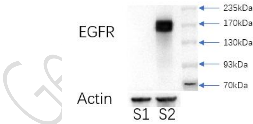
Figure 2 | The protein expression levels of Human EGFR(L858R-C797S) in the H_EGFR(L858R-C797S) BAF3 Cell Line(Cat. GM-C29678) were determined by Western blotting (WB).
